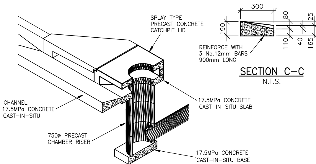
SECTION-PERSPECTIVE VIEW N.T.S.
